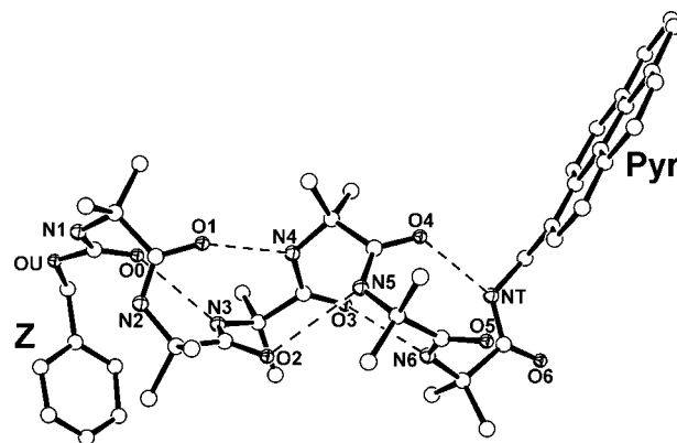
Figure 2. X-ray diffraction structure of Z-(Aib) 6 -NH-CH 2 -Pyr with partial atom numbering. The five intramolecular C=O–H–N H-bonds are indicated by dashed lines. The i \leftarrow i + 3 pattern of intramolecular H-bonds, characteristic of the 3_{10} -helix conformation, can be clearly recognized.
