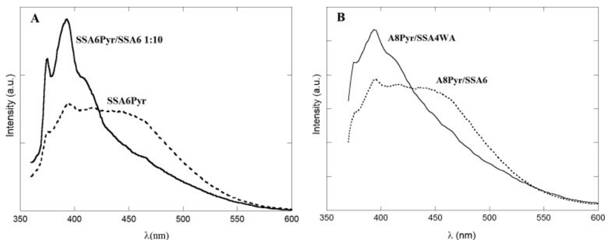
Figure 5. Fluorescence emission spectra of single- and bi-component peptide SAMs functionalized with a Pyrene chromophore on gold coated glasses. The excimer emission signals the onset of Pyr–Pyr interactions. (A) 1 : 10 SSA6Pyr/SSA6 (full line); SSA6Pyr (dotted line). (B) 1 : 1 A8Pyr/SSA4WA (full line); 1 : 1 A8Pyr/SSA6 (dotted line). All the spectra are normalized to unit area.
