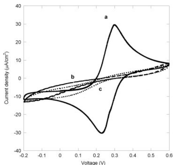
Figure 4. Cyclic voltammograms in a 0.50 mM K_3[Fe(CN)_6] aqueous solution for gold electrodes modified by the deposition of mono- (SSA4WA) and bi-component (A8Pyr/SSA4WA) peptide SAMs. The inclusion of A8Pyr in the SSA4WA SAM did not affect its packing density. Working electrode: bare gold (a, full line); gold electrode modified by SSA4WA (b, dashed line) or 1 : 1 A8Pyr/SSA4WA (c, dotted line) SAMs. Sweep rate: 50 mV/s.
